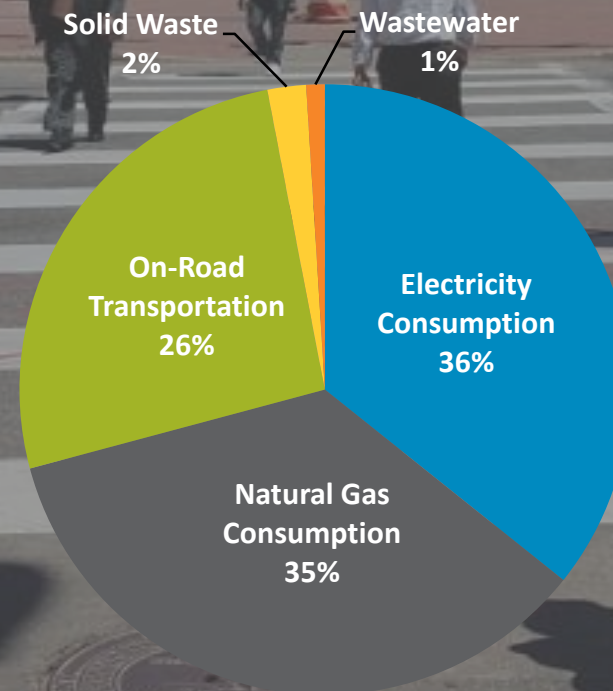
Minneapolis Greenhouse Gas Emissions by Citywide Activities (2016)
